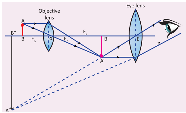
Figure 2.19 Image formation in compound microscope
